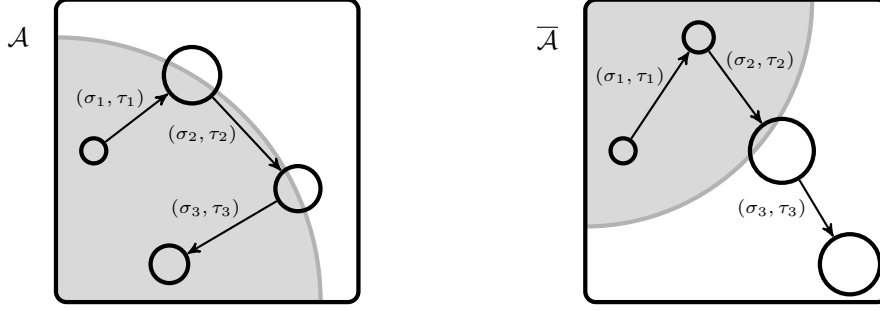
Fig. 6: Evolution of the reach-sets (depicted as circles) in \mathcal{A} (left) and \overline{\mathcal{A}} (right) after 0, 1, 2, and 3 observations. The grey areas are the states with non-empty language, i.e., \text{Reach}_{\mathcal{A}}^{\infty} and \text{Reach}_{\overline{\mathcal{A}}}^{\infty} .
