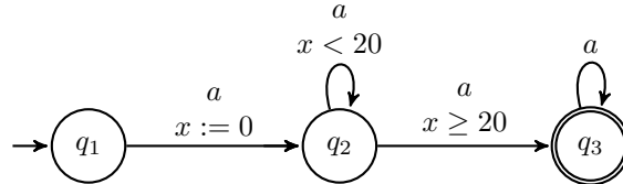
Fig. 2: TBA corresponding to F_{\geq 20}a
