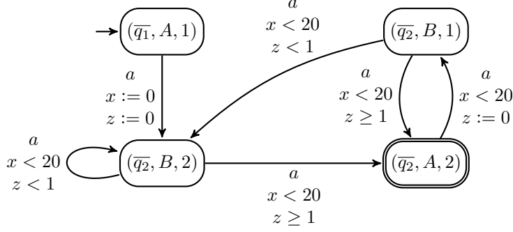
Fig. 5: TBA for the intersection of the TBA from Figure 4 (corresponding to G_{\geq 20} \text{false} ) and \mathcal{A}_D from Figure 3 (state names are as described in the construction above Lemma 1). Unreachable locations have been omitted.
