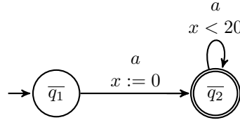
Fig. 4: TBA corresponding to G_{\geq 20} \text{false}
