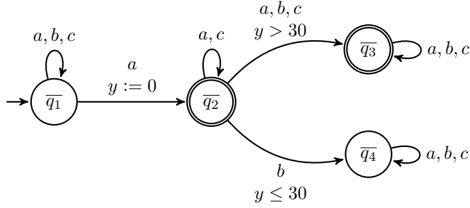
Fig. 7: TBA corresponding to F_{\ge 0}(a \wedge G_{\le 30} \neg b)
